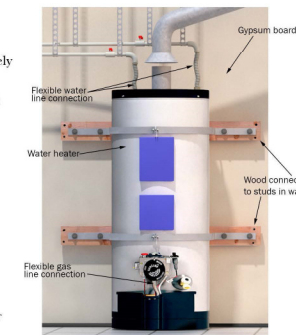
Figure G. Securing water heaters.
