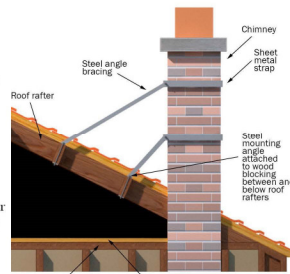
Figure C. Bracing masonry chimneys.
