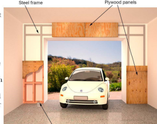
Figure B. Strengthening garage walls below living space.
